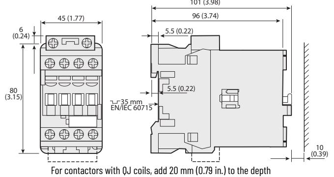
Figure 44 - 100-E26...100-E38 4-Pole Contactors with Low-consumption Coils
