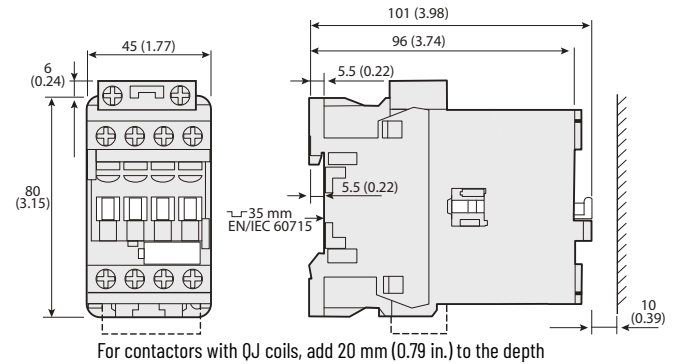
Figure 44 - 100-E26...100-E38 4-Pole Contactors with Standard Coils
