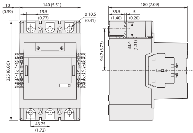
Figure 84 - 100-E265...100-E370 Contactors
