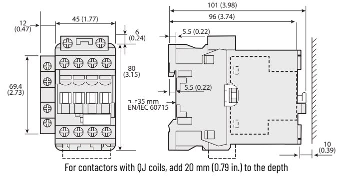
Figure 55 - 104-E26...104-E38 Reversing Contactors with Cat. No. 100-EMCA02 Mechanical and Electrical Interlock
