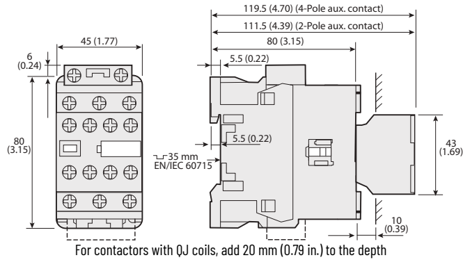
Figure 52 - 100-E26...100-E38 4-Pole Contactors with Low-consumption Coils and Front-mounted Auxiliary Contact
