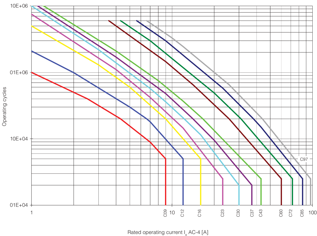
Figure 16 - AC-4, Switching of squirrel-cage motors; U_e = 230...690V
