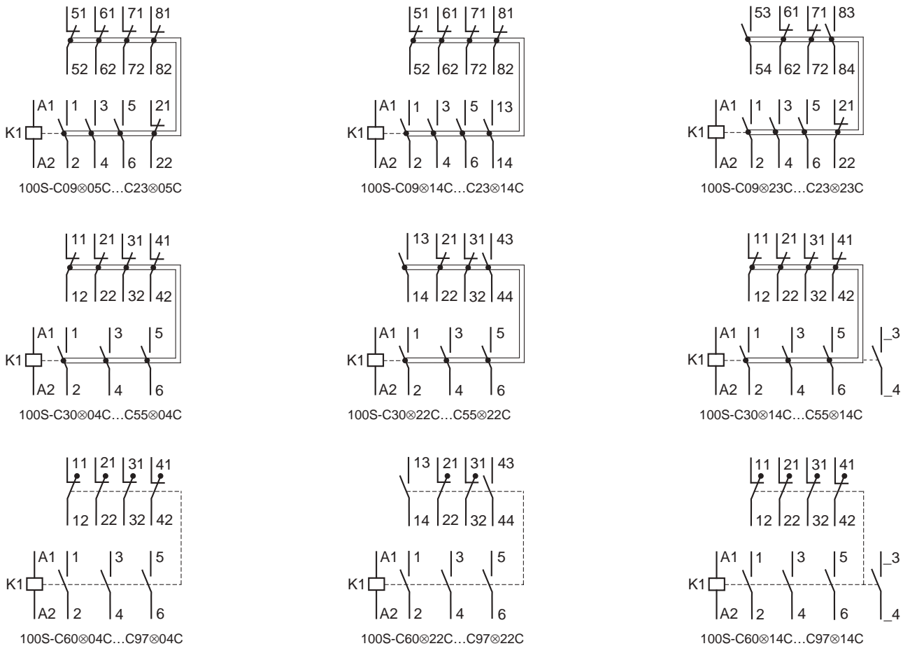
Figure 5 - Safety Contactors with 3 Main Contacts and Standard Front-mount Auxiliary Contacts
