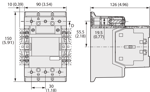
Figure 76 - 100-E116K..., 100-E146K... Contactors
