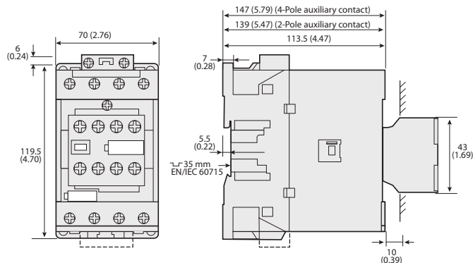
Figure 63 - 100-E40...100-E52 4-Pole Contactors with Front-mounted Auxiliary Contact
