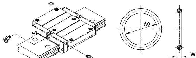
O Ring
