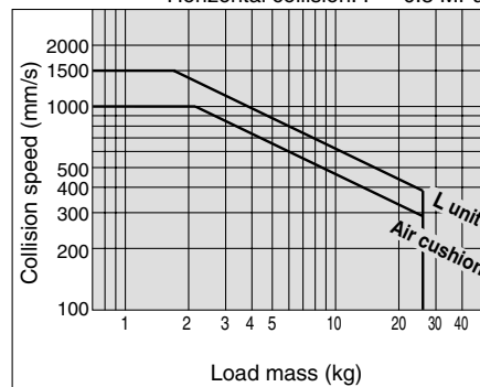
ø20 Horizontal collision: P = 0.5 MPa
