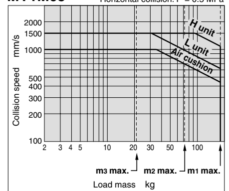
MY1M63 Horizontal collision: P = 0.5 MPa
