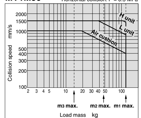
MY1M50 Horizontal collision: P = 0.5 MPa
