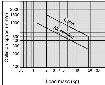
ø16 Horizontal collision: P = 0.5 MPa
