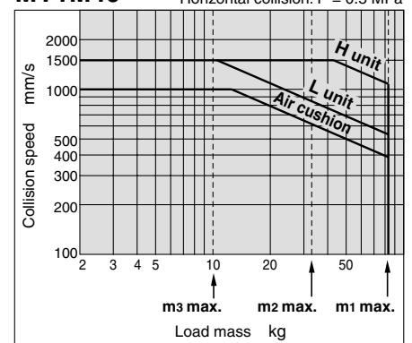
MY1M40 Horizontal collision: P = 0.5 MPa
